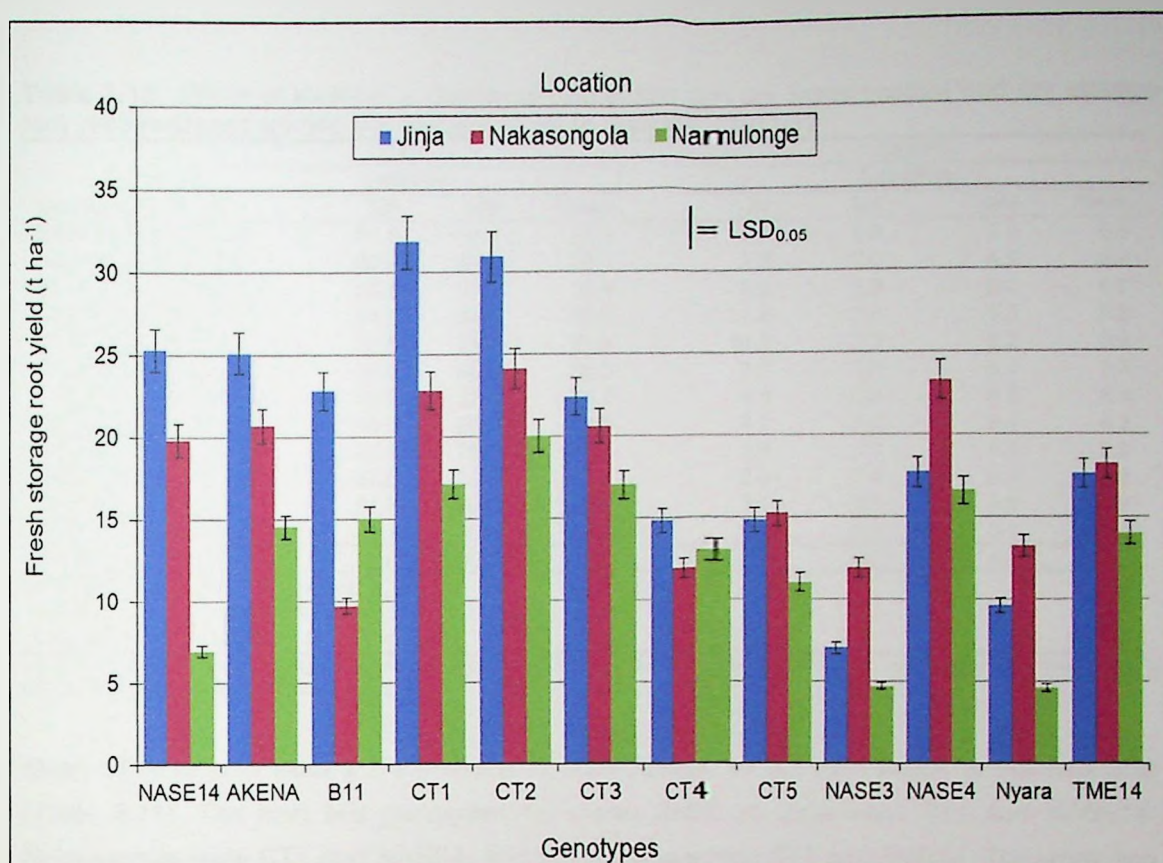
Figure 3.4: Fresh storage root yield ( \text{t ha}^{-1} ) of 12 cassava genotypes evaluated at three locations averaged across five harvest times in Uganda, 2011/12
