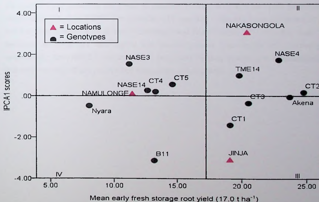
Figure 4.1: Biplot of mean early fresh storage root yield and IPCA1 scores for 12 cassava genotypes evaluated nine months after planting at three locations in Uganda.
