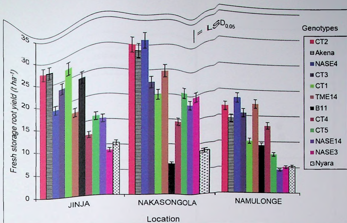
Figure 4.2: Mean performance in early fresh storage root yield ( t\ ha^{-1} ) of 12 genotypes evaluated nine months after planting at three locations in Uganda.
