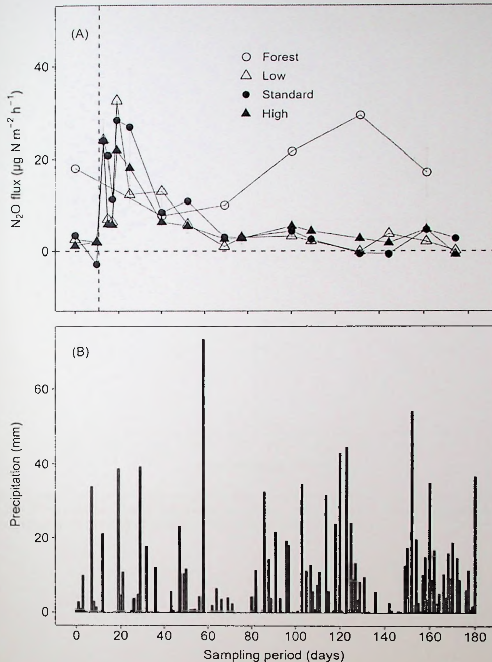
Appendix F.1. (A) Mean ( \pm standard error, SE, n = 4 ) soil N_2O fluxes measured between May and October 2019 from the reference forest plots and replicate treatment plots of the completely randomized design (CRD) experiment established in the 20-year-old sugarcane plantation, and (B) the bars represent the daily precipitation measured between May and October 2019 from both the reference forest plots and sugarcane plots. The dashed vertical blue line indicates the timing of the application of the single combined dose of urea and muriate of potash fertilizers in the sugarcane. The dashed horizontal line indicates the background level of the soil N_2O fluxes from both the reference forest and sugarcane plots. Standard equals 70 kg N + 23 kg K ha^{-1} growth cycle -1 , low equals 0.5 times standard and high equals 1.5 times standard.
