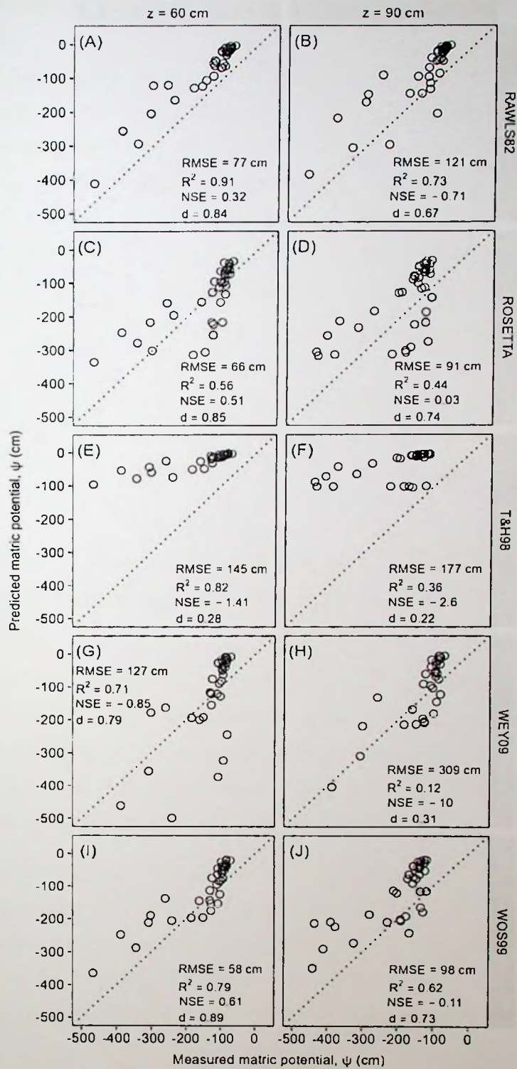
Figure 4.4. Predicted and measured soil matrix potential based on RAWLS82 (A and B), ROSETTA (C and D), T&H98 (E and F), WEY09 (G and H), and WOS99 (I and J) pedotransfer functions at soil depths of 60 and 90 cm. The corresponding root mean square error (RMSE), coefficient of determination ( R^2 ), Nash Sutcliffe efficiency (NSE), and index of agreement ( d ) are reported in each subplot.
