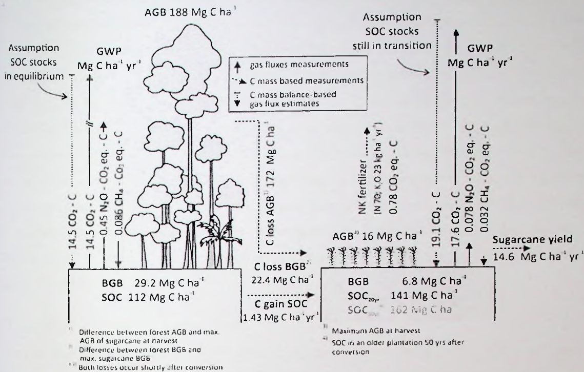
Figure 5.1. Schematic illustration of the implication of forest replacement with fertilizer-based sugarcane production on the net ecosystem C fluxes. AGB is aboveground biomass, BGB is belowground biomass, SOC 20 yr , and SOC 50 yr are the soil organic carbon stocks in the sugarcane fields after 20 and 50 years of establishment (deforestation), respectively. The fertilizer application rates, maximum AGB, and yield for the sugarcane system represent a typical standard sugarcane system (i.e., Standard equals 70 kg N + 23 kg K ha -1 growth cycle -1 ) in north-western Uganda.
