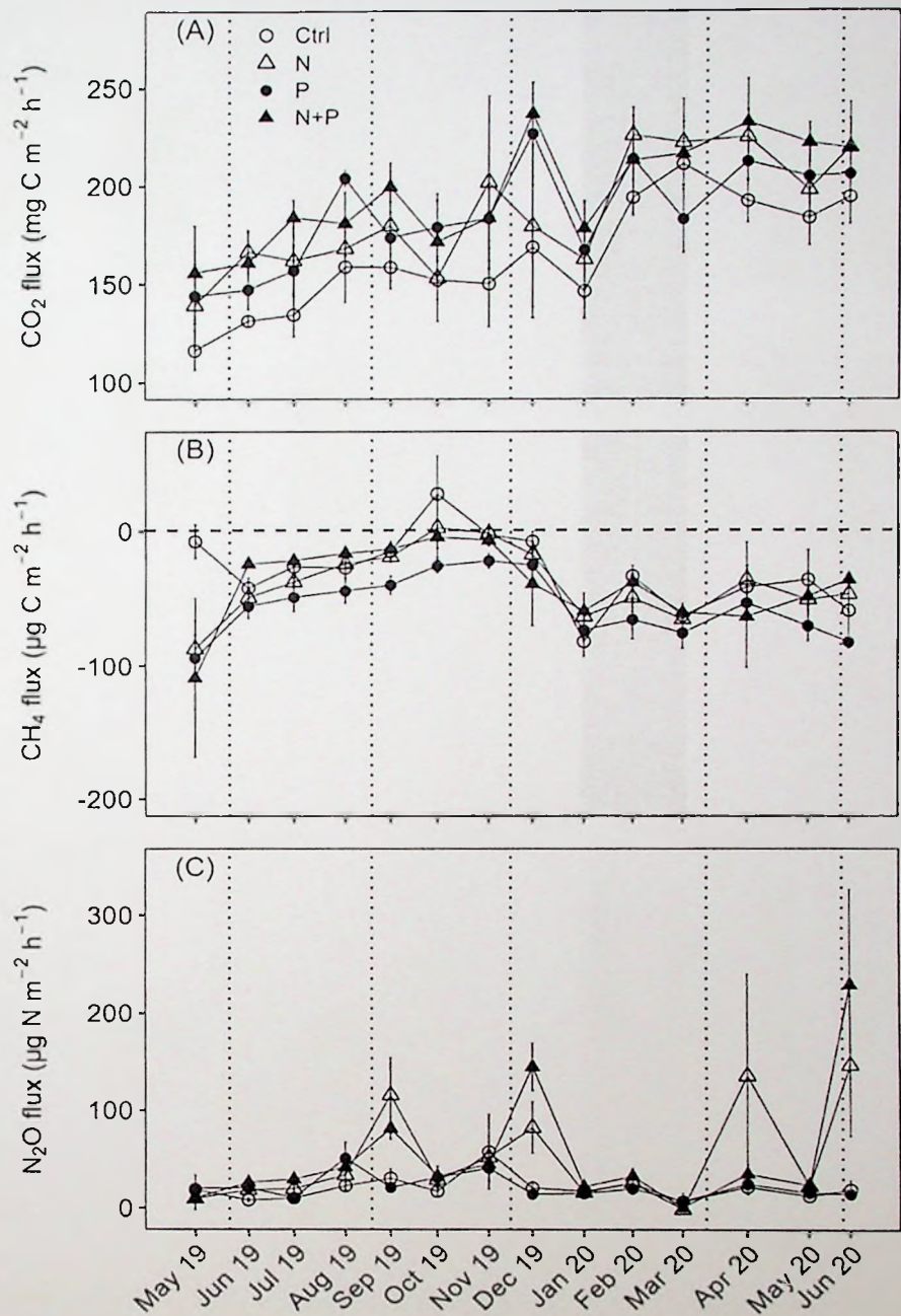
Figure 2.4. Mean ( \pm standard error, SE, n = 4 ) soil CO 2 fluxes (A), CH 4 fluxes (B), and N 2 O fluxes (C) measured monthly (between May 2019 and June 2020) from control (Ctrl), nitrogen (N), phosphorus (P), and N + P plots of the nutrient manipulation experiment. Vertical lines indicate the timing of each split dose of N (31.3 kg N ha -1 ), P (12.5 kg P ha -1 ), and N (31.3 kg N ha -1 ) + P (12.5 kg P ha -1 ) fertilization every 3 months. The gray-shaded rectangle marks the beginning and end of the dry season (January and February; monthly precipitation < 100 mm). Note: transitory N 2 O fluxes (measured within 28 days from fertilization) from N addition plots (N and N + P) were detrended to compensate for the absence of frequent measurements immediately after fertilization coming from sampling GHG fluxes monthly.
