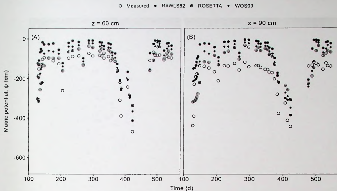
Appendix F.5. Predicted matric potential with ROSETTA, RAWLS82, and WOS99 PTFs and the measured soil matric potential at soil depths of 60 (A) and 90 cm (B) between May 2019 and June 2020.
