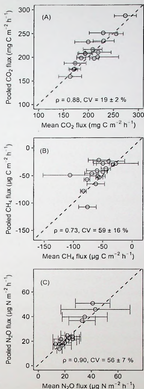
Figure 2.1. Comparison of the soil CO 2 fluxes (A), soil CH 4 fluxes (B), and soil N 2 O fluxes (C) from pooled sampling and the mean of four chamber measurements for the month of February 2020 in the Budongo Central Forest Reserve. \rho is the Spearman correlation coefficient, and CV is the coefficient of variation. Error bars are derived from standard error of the mean.
