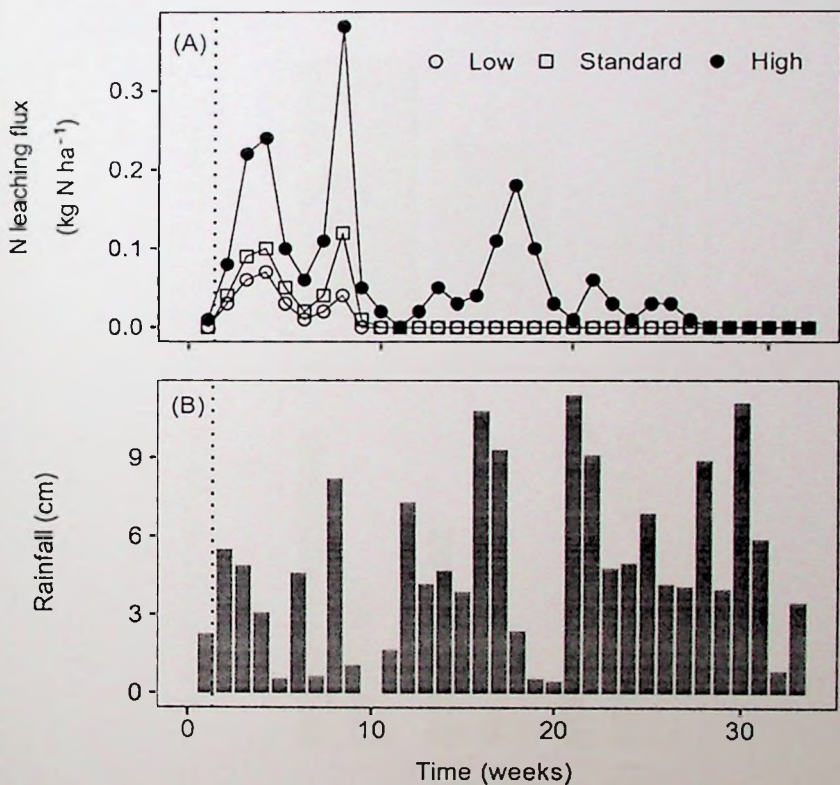
Figure 4.6. (A) Mean weekly N leaching flux from low, standard, and high fertilization regimes and (B) weekly rainfall sums between April and December 2019. The vertical dotted line indicates the timing of a single-dose fertilizer application in the treatment plots.
