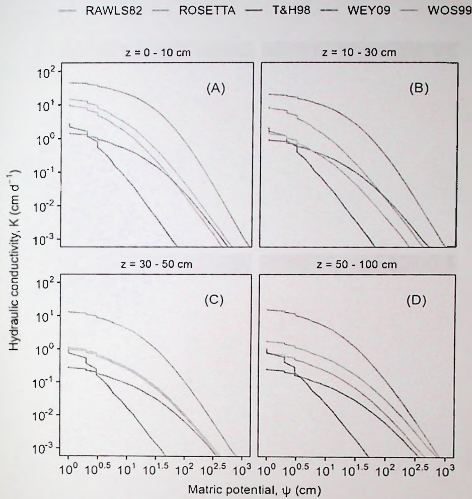
Appendix F.3. Soil hydraulic conductivity curve at four different soil depths (0-10 cm—A; 10-30 cm—B; 30-50 cm—C; and 50-100 cm—D) based on soil hydraulic parameters of the van Genuchten model ( \theta_r , \theta_s , \alpha , and n ) and saturated hydraulic conductivity, K_s , estimated using five PTFs (RAWLS82, ROSETTA, T&H98, WEY09, and WOS99).
