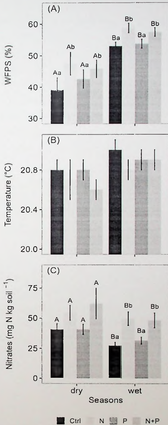
Figure 2.2. Mean ( \pm standard error, SE, n = 4 ) WFPS (A), soil temperature (B), and nitrates (C) in the top 0.05 m of the control (Ctrl), nitrogen (N), phosphorus (P), and N + P plots of the nutrient manipulation experiment measured during the dry (January and February; monthly precipitation < 100 mm) and wet (March to December; monthly precipitation > 100 mm) seasons. Different lowercase letters indicate significant differences between treatments and the control, while different uppercase letters indicate significant differences between seasons (LMEMs; p \leq 0.05 ).
