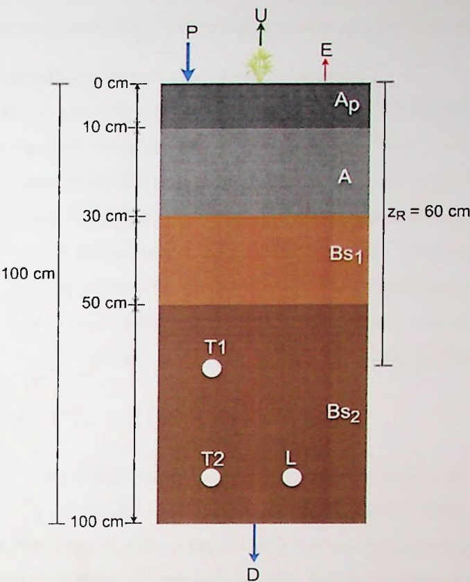
Figure 4.2. Sketch of the 1-m-deep soil profile composed of four soil layers (Ap, A, Bs1, Bs2 corresponding to 0-10 cm, 10-30 cm, 30-50 cm, and 50-100 cm soil depths, respectively). Precipitation (P) and evaporation (E) occur at the soil surface. At the same time, the sink term U controls transpiration through the roots in the root zone ( z_R=60 cm), and water moves down across the bottom of the soil profile through drainage (D). T1 and T2 are the observation nodes ( z=60 cm and z=90 cm) at which simulated and measured matric potential values were compared to test pedotransfer function performance.
