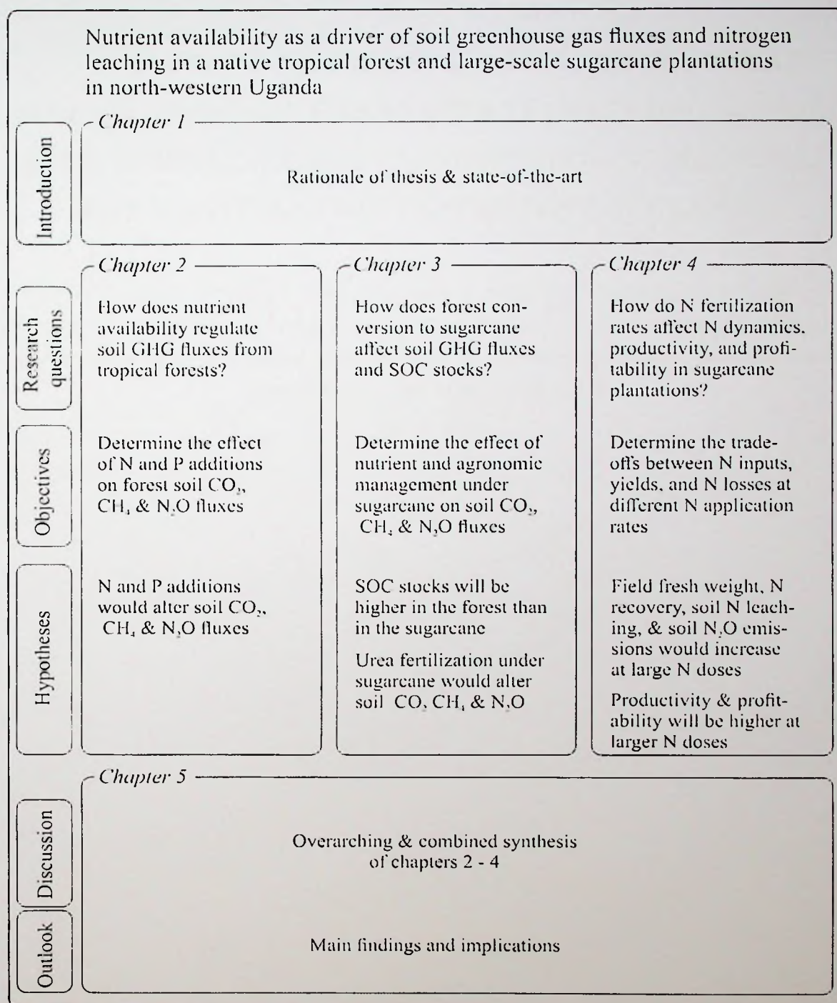
Figure 1.1. PhD conceptual flow diagram
