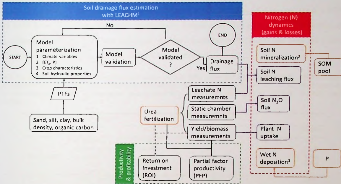
Figure 4.3. Flow chart of the methodology underpinning the study comprising of 1 drainage flux estimated with water subroutine of the Leaching Estimation and Chemistry Model (LEACHM; blue box; Hutson, 2003); nitrogen dynamics estimation (red box); and productivity and profitability assessment (green box). P denotes precipitation, and ET_p means potential evapotranspiration estimated with the Penman-Monteith method (Allen et al., 1998). PTFs means pedotransfer functions (RAWLS82, ROSETTA, T&H98, WEY09, and WOS99) used to estimate the soil hydraulic properties in each soil layer in the 1-m-deep soil profile. N_2O and SOM denote nitrous oxide emissions and soil organic matter, respectively. 2 Soil N mineralization was estimated from SOM using an empirical relationship proposed by R. H. McKenzie, personal communication, February 23, 2017. 3 Wet N deposition in precipitation estimated by (Manu et al., 2022). Brown boxes and arrows represent N gains, while purple boxes and arrows represent N losses.
