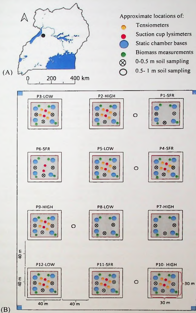
Figure 4.1. (A) Geographic location of the study area (black dot) in the north-western part of Uganda, (B) sketch of the completely randomized design (CRD) experiment set up in a 5.6 ha field. The CRD experiment consisted of 12 treatment plots (measuring 40 m × 40 m) in which soil matric potential, nitrate concentrations, and soil nitrous oxide fluxes, were measured using tensiometers (yellow circles), suction cup lysimeters (red circles), and static chamber bases (blue circles), respectively, under standard (SFR; 70 kg ha -1 ), low (0.5 times SFR), and high (1.5 times SFR) nitrogen (N) applications. The plots are labelled by reporting plot (P) number and four replications of N applications (LOW, SFR, HIGH). Biomass measurements (green circles) and soil sampling between 0 and 0.5 m (black crossed circle) were carried out in each treatment plot, while deep soil sampling (0.5 – 1.0 m; empty black circles) are located between the treatment plots.
