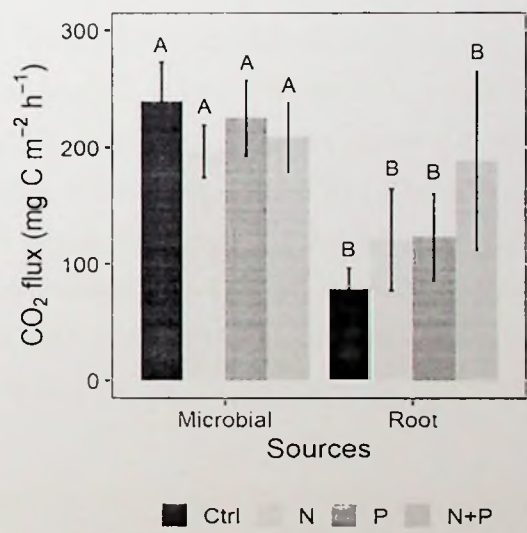
Figure 2.6. Mean (± standard error, SE, n = 4) soil CO 2 flux from the control (Ctrl), nitrogen (N), phosphorus (P), and N + P plots of a trenching treatment separated into microbial and root sources. Different upper-case letters indicate significant differences between microbial and root contribution to total CO 2 efflux (linear mixed effects models; p ≤ 0.05).
