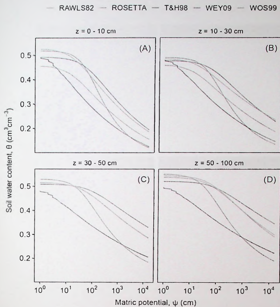
Appendix F.2. Soil water retention curves at four different soil depths (0-10 cm—A; 10-30 cm—B; 30-50 cm—C; and 50-100 cm—D) based on soil hydraulic parameters of the van Genuchten model ( \theta_r , \theta_s , a , and n ) estimated using five PTFs (RAWLS82, ROSETTA, T&H98, WEY09, and WOS99).
