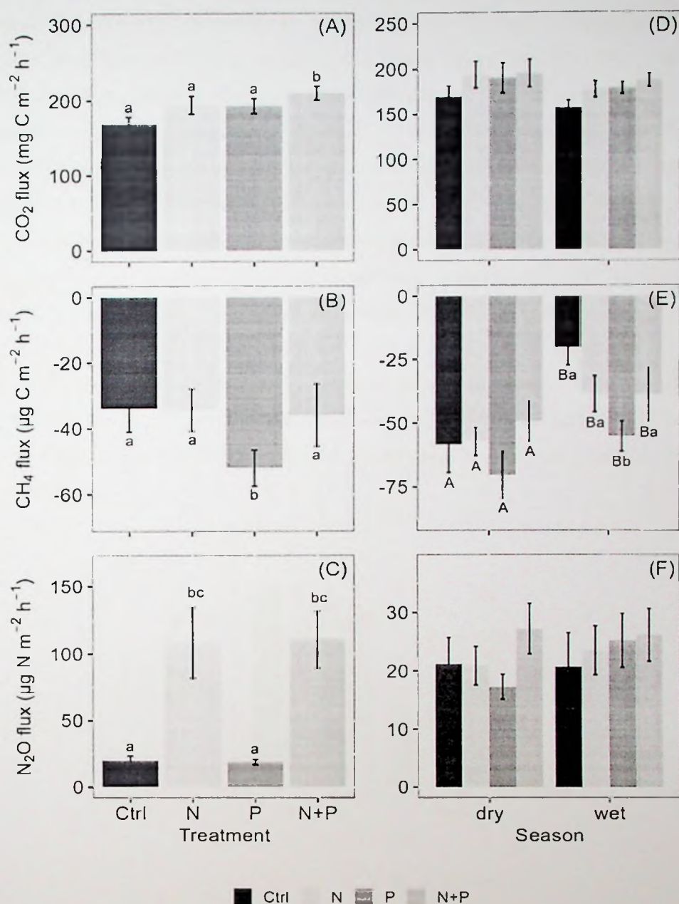
Figure 2.5. Mean ( \pm standard error, SE, n = 4 ) soil \text{CO}_2 fluxes (A, D), \text{CH}_4 fluxes (B, E), and \text{N}_2\text{O} fluxes (C, F) from the control (Ctrl), nitrogen (N), phosphorus (P), and N + P plots of the nutrient manipulation experiment. Column 1 (A–C) includes only fluxes measured during the transitory phase (0–28 days after fertilization), and all the transitory fluxes were in the wet season (monthly precipitation > 100 mm). Column 2 (D–F) includes only background-level fluxes (fluxes measured more than 28 days after fertilization). Different lowercase letters indicate significant differences between nutrient addition treatments and the control, while different uppercase letters indicate significant differences between seasons (linear mixed effects models; p \leq 0.05 ). Note: transitory \text{N}_2\text{O} fluxes (measured within 28 days from fertilization) from N addition plots (N and N + P) were detrended to compensate for the absence of frequent measurements immediately after fertilization coming from sampling GHGs monthly.
