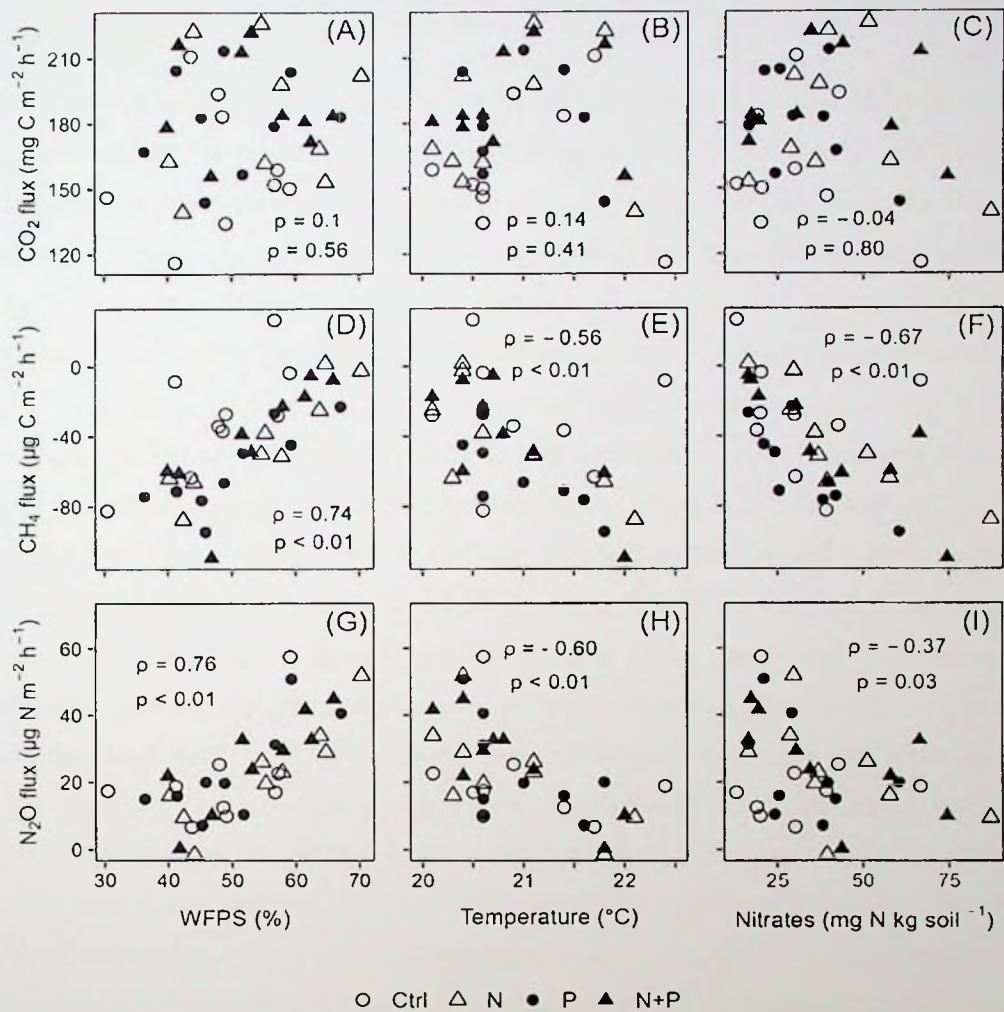
Figure 2.7. The Spearman correlation coefficient between mean background CO 2 (A–C), CH 4 (D–F), and N 2 O (G–I) fluxes and WFPS (column 1), soil temperature (column 2), and nitrates (column 3) using monthly measurement means of four replicate treatment plots (i.e., control (Ctrl), nitrogen (N), phosphorus (P), and N + P) taken between May 2019 and June 2020 ( p \leq 0.05 ; n = 16 ; i.e., four replicate plots in each of the four treatments). \rho is Spearman's correlation coefficient.
