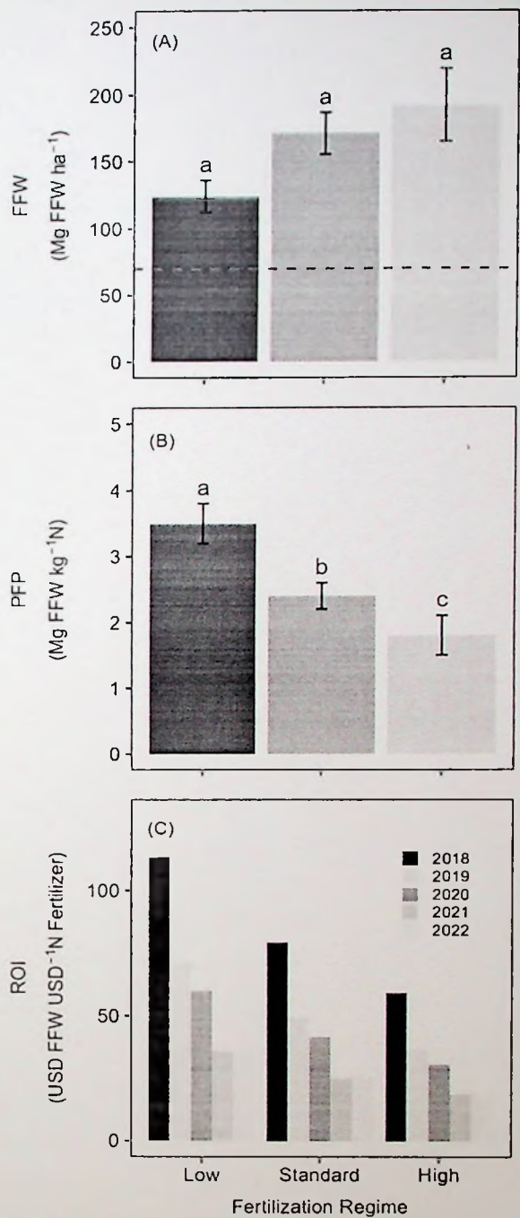
Figure 4.7. Mean ( \pm standard error, SE, n = 4 ) yield expressed as field fresh weight (FFW; A), partial factor productivity (PFP; B), and return on investment (ROI; C), along the fertilizer intensification gradient (low, standard, and high). Lowercase letters in panels A, B, and C indicated significant differences between treatments (ANOVA with Tukey's HSD test with a multiple-comparison extension test at p \leq 0.05 ). The dotted horizontal red line in panel A indicates the minimum acceptable FFW from sugarcane ratoon fields in north-western Uganda, below which sugarcane fields are plowed down and new ones established (based on Masindi Sugarcane Farmers' Association).
