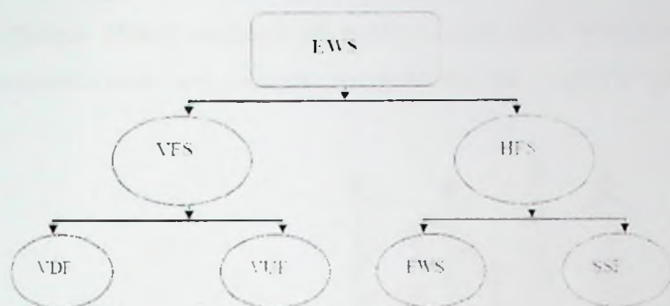
Figure 2. 6: Schematic classification of engineered/constructed wetland systems (source: Mbuligwe et al. , 2011). EWS = engineered wetland systems; VFS = vertical flow wetland systems; HFS = horizontal flow wetland systems; VDF = Vertical downward flow wetland systems; VUF = vertical upward flow wetland systems; FWS = free water surface wetland system; SSF = sub-surface flow wetland system.
