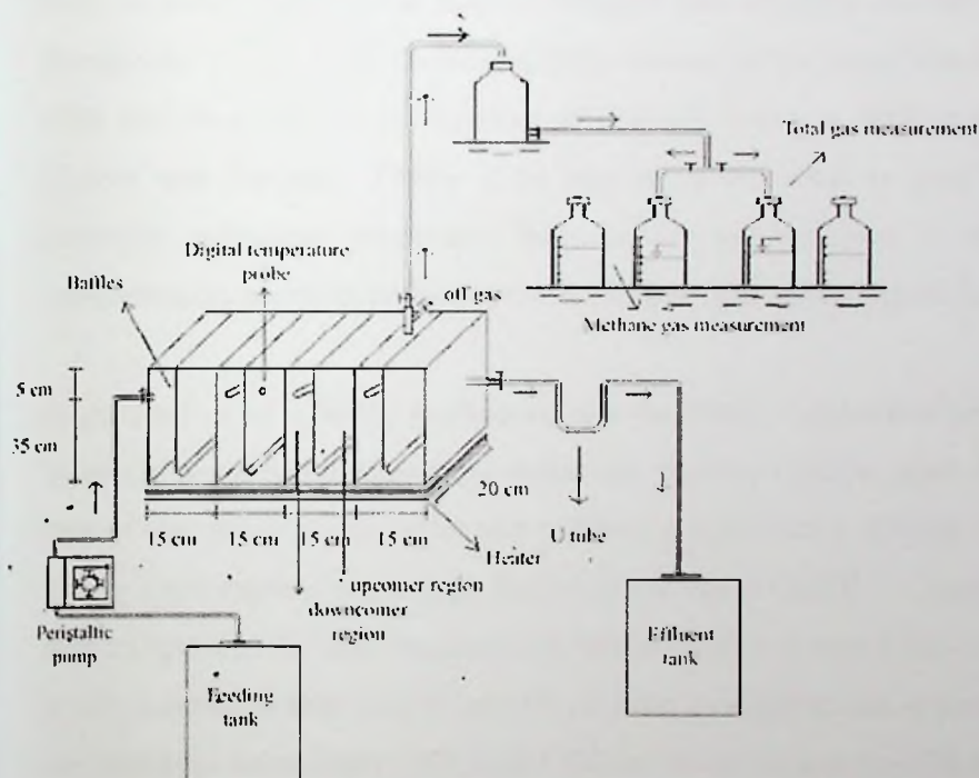
Figure 2. 5: Schematic diagram of the anaerobic baffled reactor (ABR) (source: Kuşçu and Sponza, 2005)
