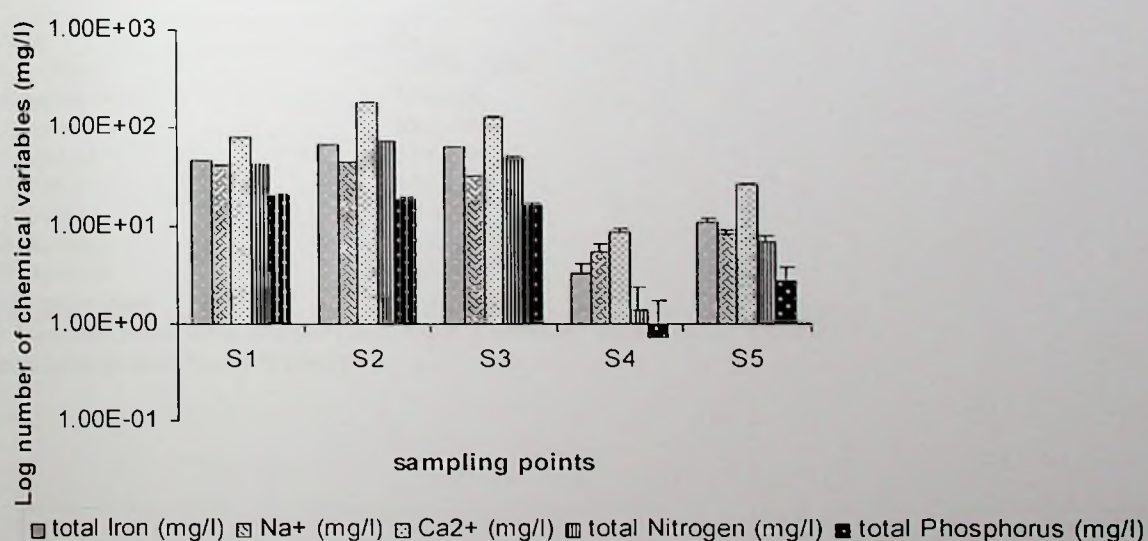
Figure 4. 1: Mean concentrations of chemical parameters of sugar processing effluent, distillery effluent and R. Musamya water
