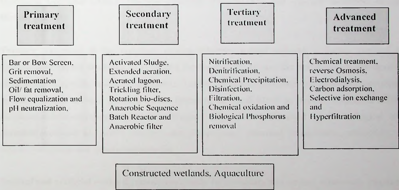
Figure 2. 1: Wastewater treatment categorization and technologies. Source: Schölzel and Bower, (1999)
