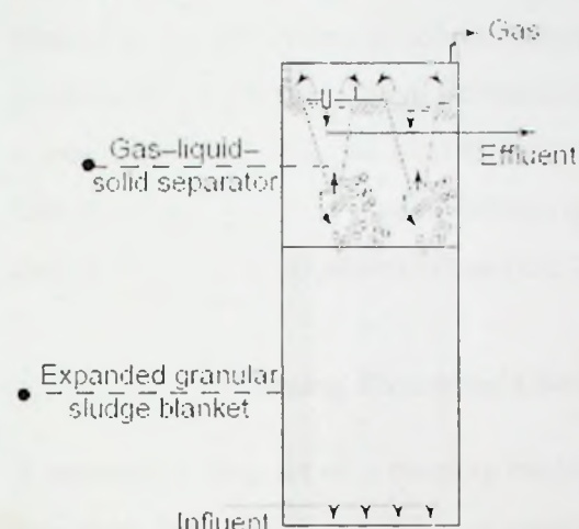
Figure 2. 3: Expanded granular sludge blanket (source: Nicoletta et al., 2000)
