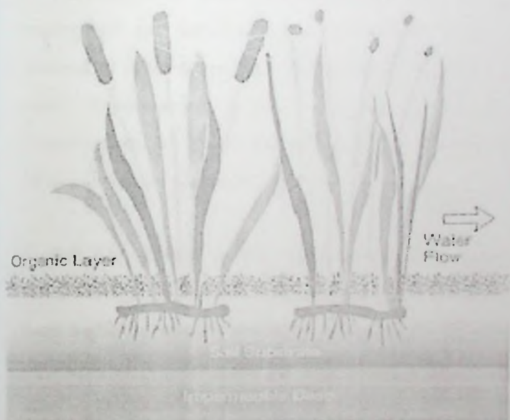
Figure 2. 8: Free Water Surface Constructed Wetland (source: Oketch, 2006)
