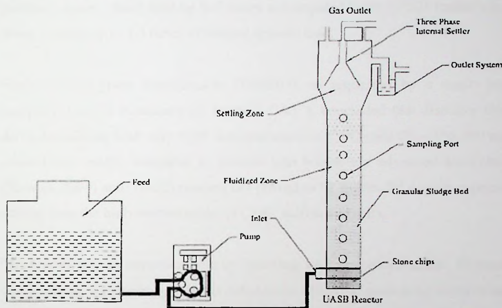
Figure 2. 2: Upflow anaerobic sludge blanket reactor (UASB) reactor (source: Rajeshwari et al., 2000).
