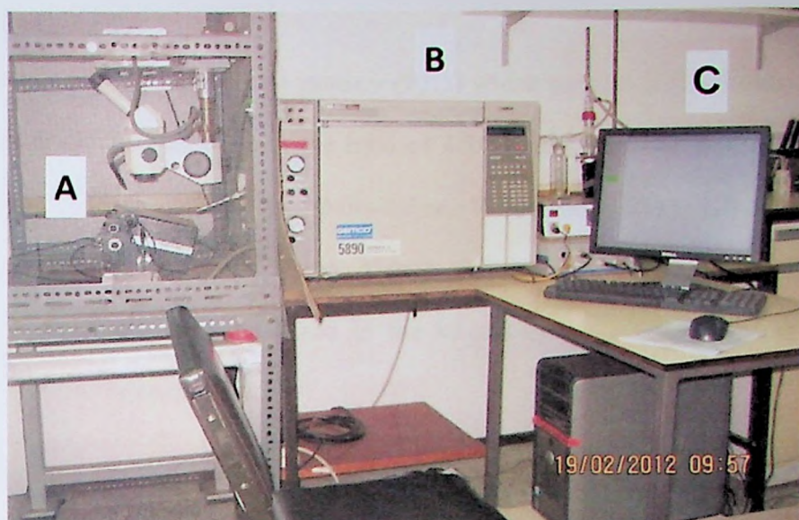
Figure 6.3 Gas chromatography-electroantennographic detection apparatus A, Electroantennographic detector; B, Gas chromatograph, Computer screen. Photo: Egonyu J.P.
