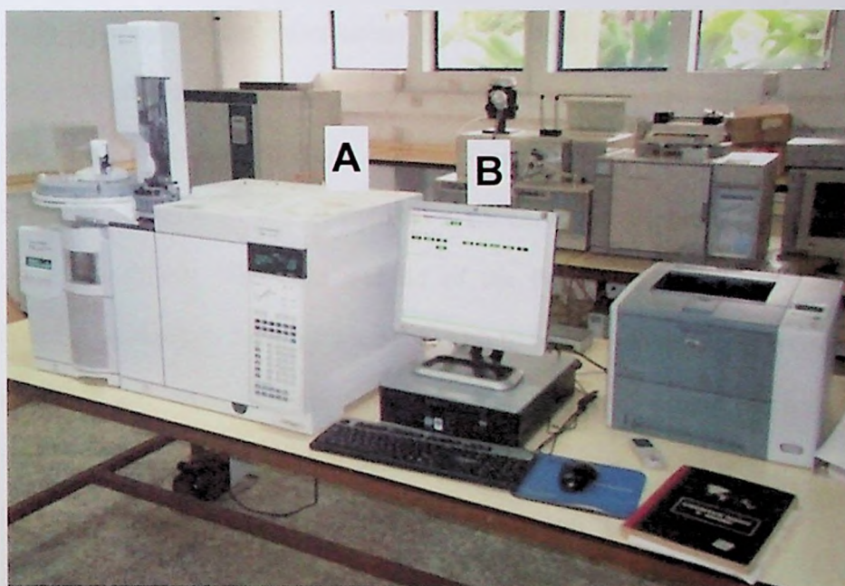
Figure 6.4 Gas chromatography-mass spectrometry apparatus A, Gas chromatograph, Computer screen. Photo: Egonyu J.P.
