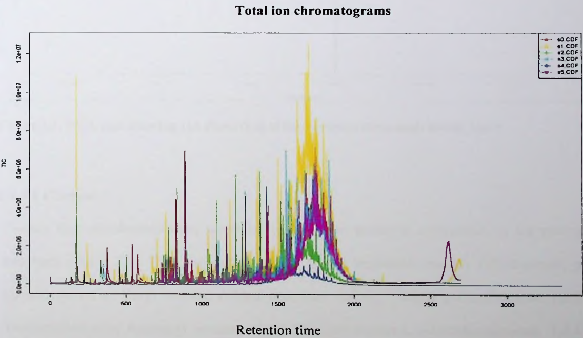
Figure 3.1. Generated total ion chromatograms for secondary metabolites from cymbopogon ( S_1 ), desmodium ( S_2 ), NERICA 1 rice ( S_3 ), mucuna ( S_4 ) maize ( S_5 ) and control ( S_0 ) overlayed. TIC = Total Ion Chromatograms. CDF = Computable Document Format
