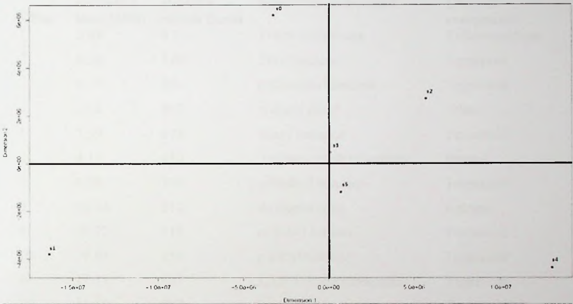
Figure 3.2: PCA plot showing the clustering of the various compounds under study
