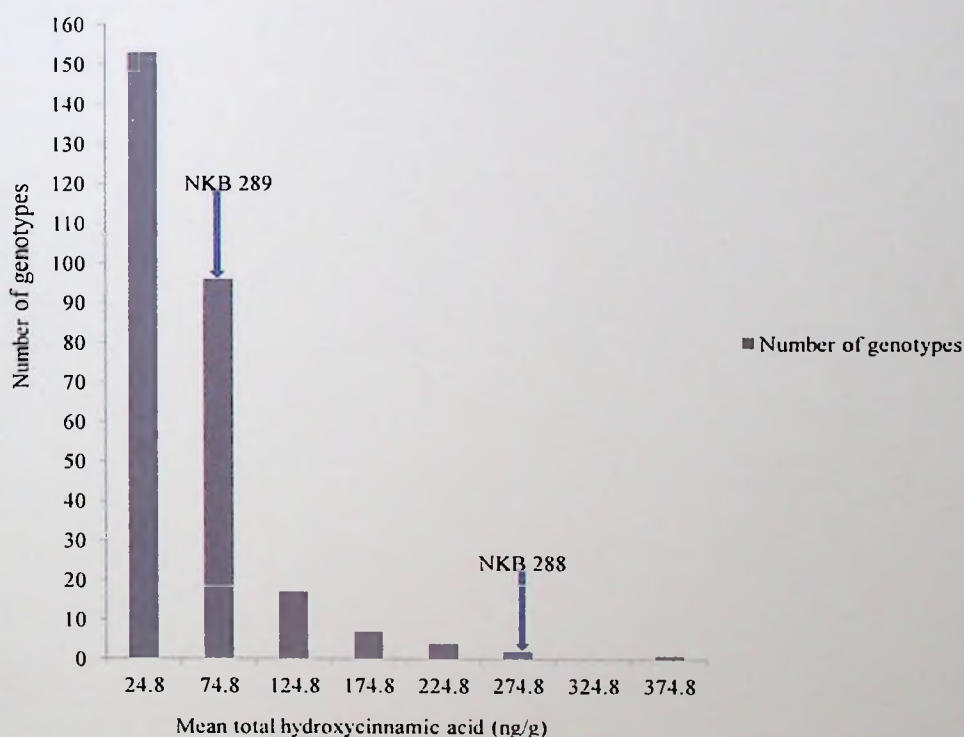
Figure 8.7. Mean total hydroxycinnamic acid (ng/g) in the segregating population of New Kawogo (NKB288) and Beauregard (NKB289).
