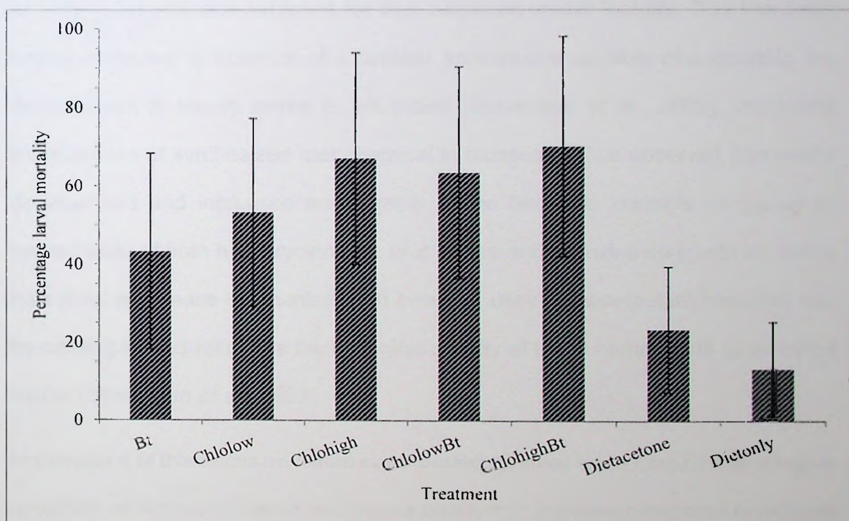
Figure 7.4 Mean mortality ( \pm SEM) of C. puncticollis and C. brunneus larvae feeding on diets treated with 5-O-caffeoylquinic acid and Bt toxins.
