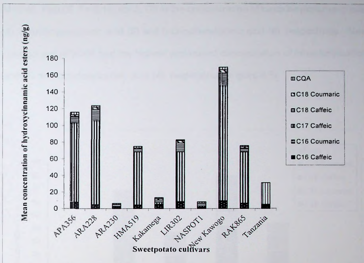
Figure 4.4 Mean concentration of hydroxycinnamic acid esters in the root epidermal tissues of selected sweetpotato varieties.
