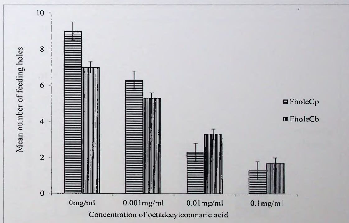
Figure 5.2 Mean number of feeding holes produced by C. puncticollis and C. brunneus on sweetpotato root plugs treated with octadecyl coumaric acid, N=15 , SEM.
