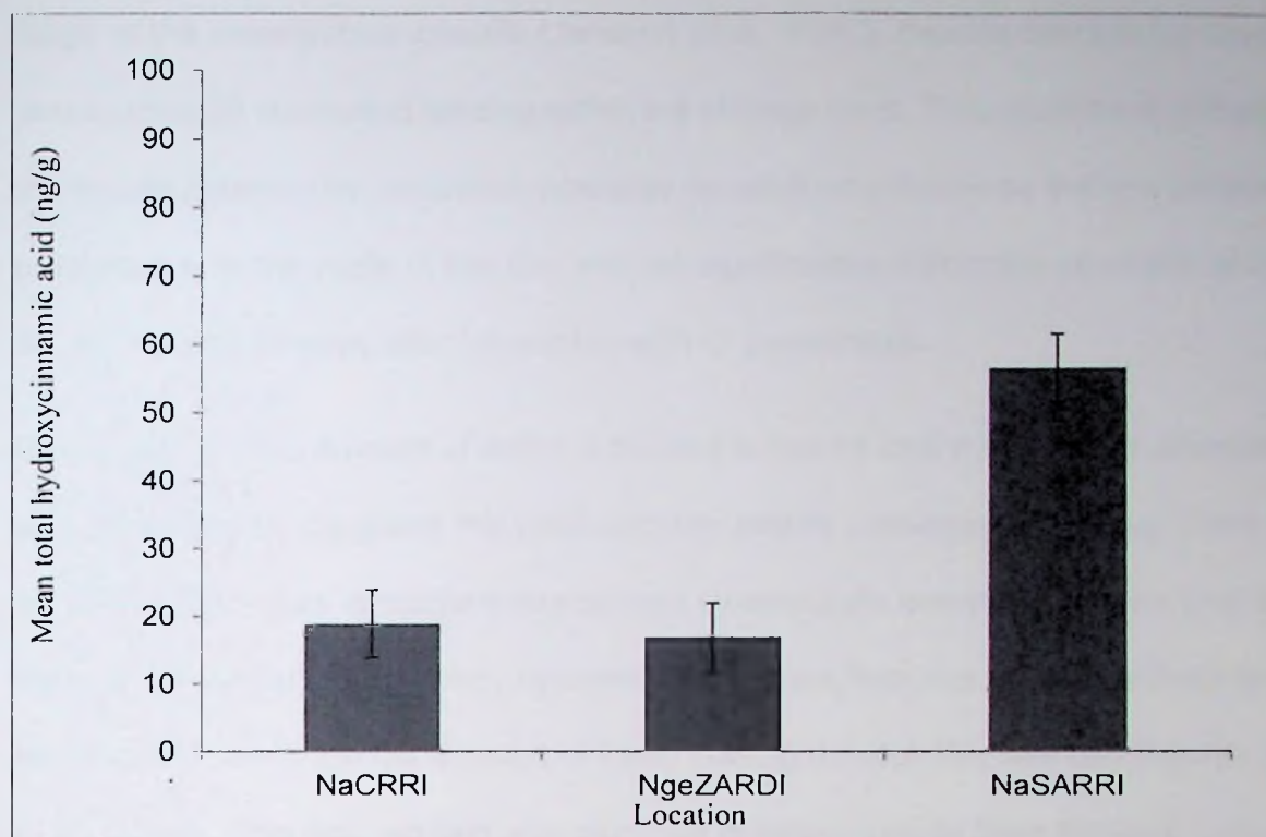
Figure 8.8 Mean total hydroxycinnamic acid (ng/g) ( \pm SEM) in the roots a segregating population of New Kawogo and Beauregard across locations
