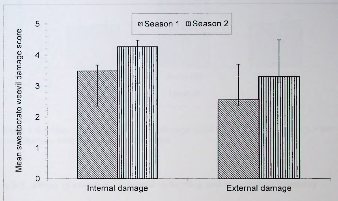
Figure 8.4 Mean sweetpotato damage score ( \pm SEM) on the internal and external stem base of sweetpotato vine in two seasons.
