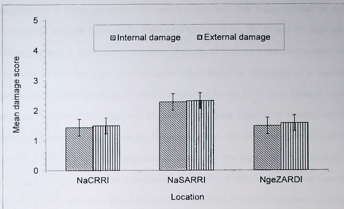
Figure 8.5 Mean sweetpotato weevil damage ( \pm SEM) on the stem base portion of sweetpotato vine recorded at 3 locations.
