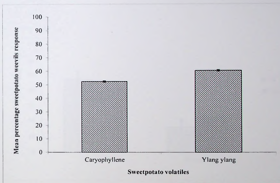
Figure 6.5. Mean percentage attraction of sweetpotato weevils to caryophyllene and ylang ylang (n=20, replicated 5 times).
