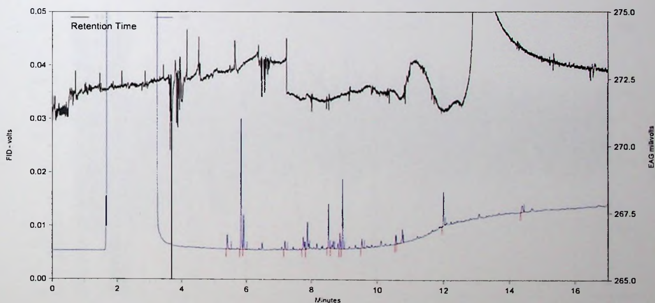
Figure 6.11. Chromatograms of New Kawogo volatiles plus pheromone and EAG response using a male C. puncticollis antenna with the tip cut and the second antenna removed
