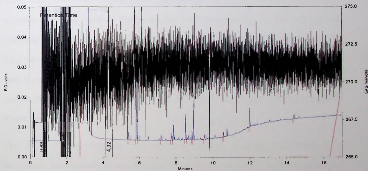
Figure 6.13. Chromatograms of New Kawogo volatiles plus pheromone and EAG response using a C. puncticollis antenna with the tip cut and the second antenna removed.
