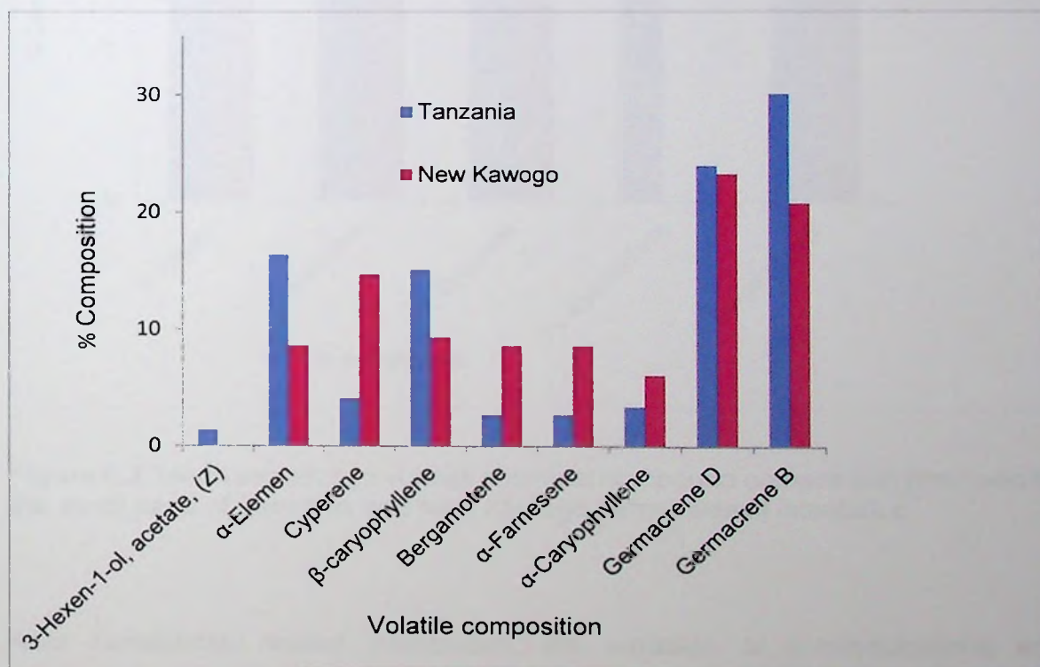
Figure 6.2. Mean percentage volatile chemical compound composition produced by the storage root of Tanzania and New Kawogo after weevil infestation
