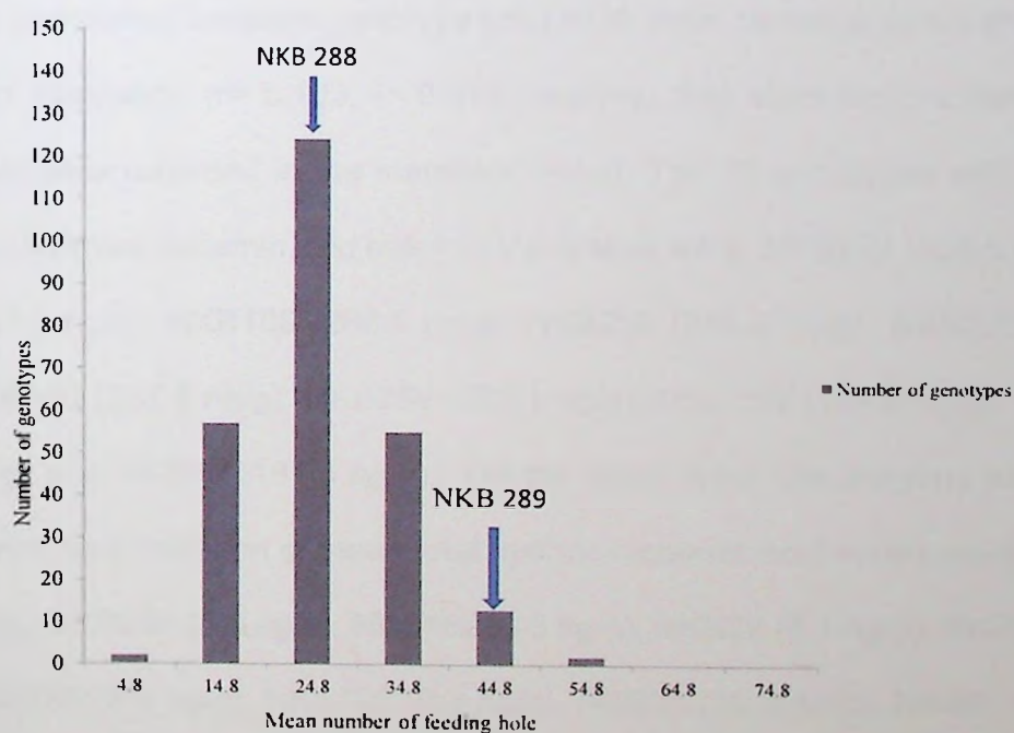
Figure 8.6 Mean number of feeding holes in a segregating population of New Kawogo (NKB288) and Beauregard (NKB289).
