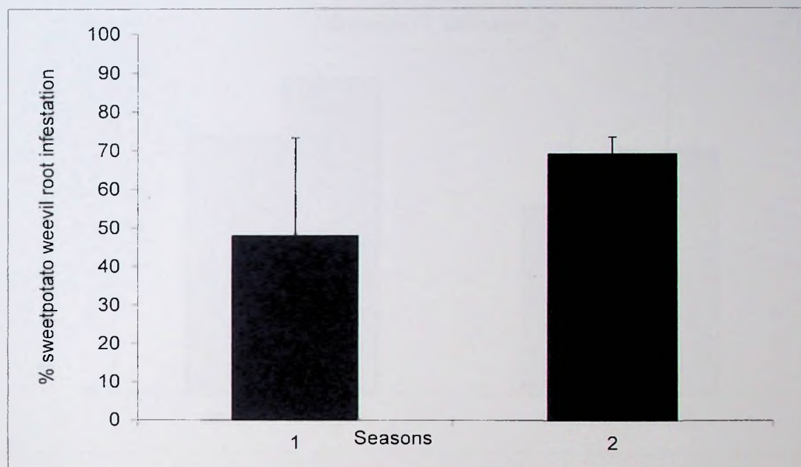
Figure 8.3 Mean percentage ( \pm SEM) sweetpotato weevil root infestation across seasons
