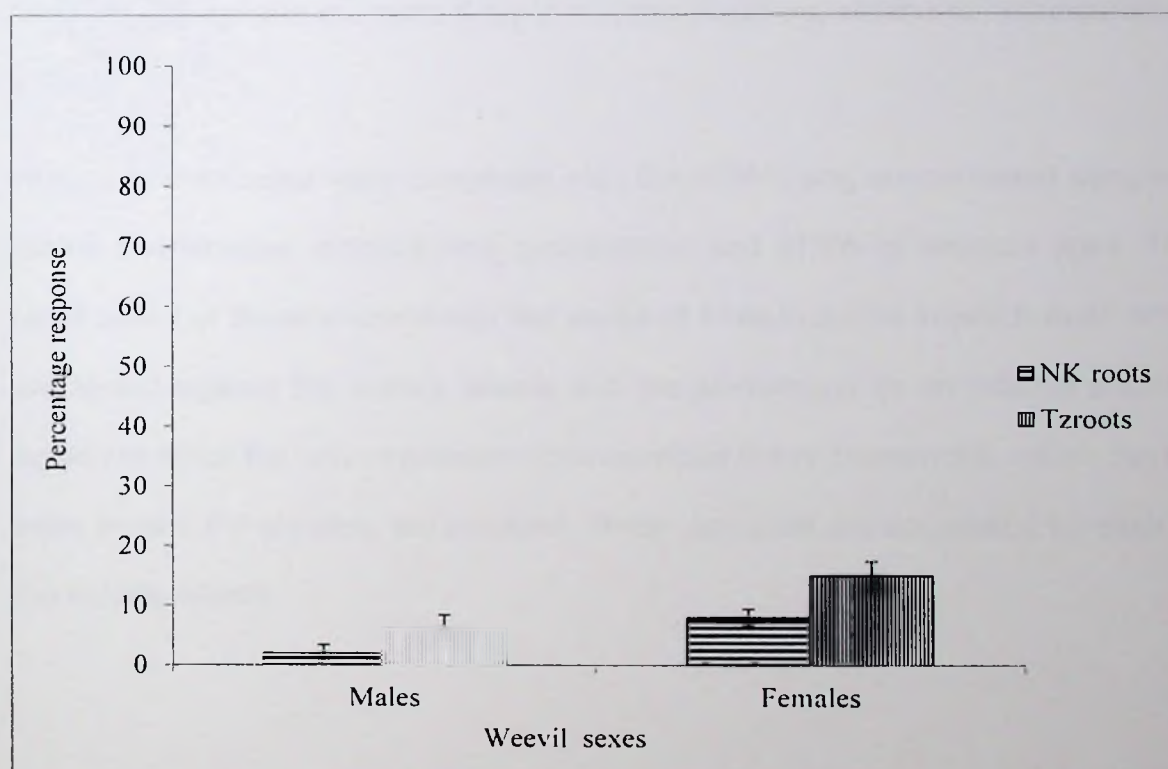
Figure 6.7. Mean attraction of male and female sweetpotato weevil to sweetpotato root odours ( n=20 , replicated 5 times) of New Kawogo (NK) and Tanzania (Tz).
