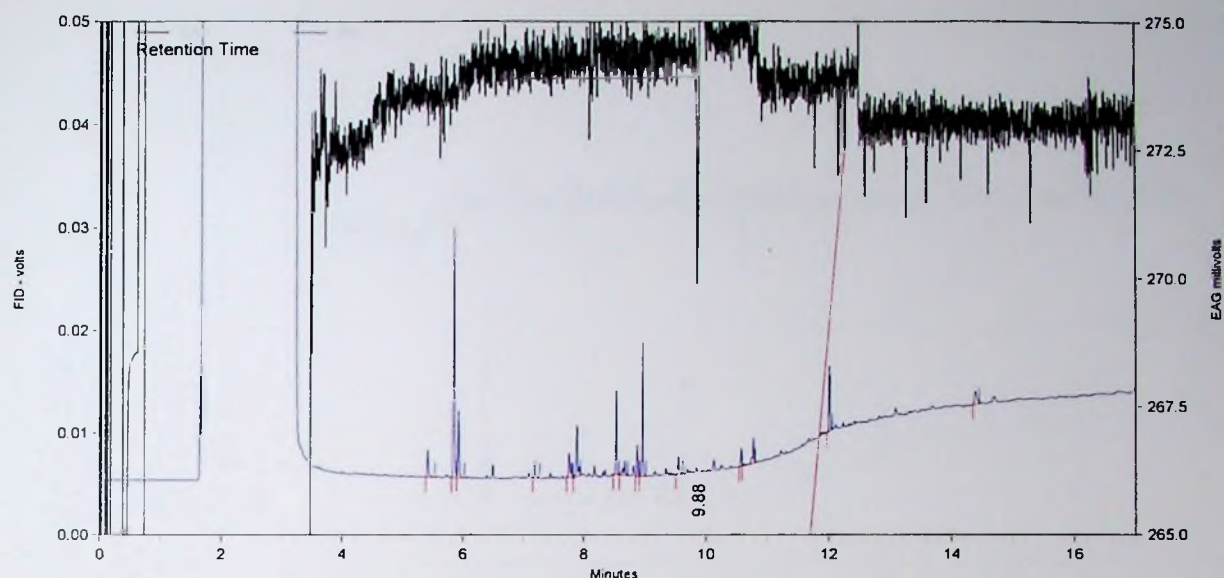
Figure 6.10. Chromatograms of Tanzania volatiles plus pheromone and EAG response using a male C. puncticollis antenna with the tip cut and the second antenna removed
