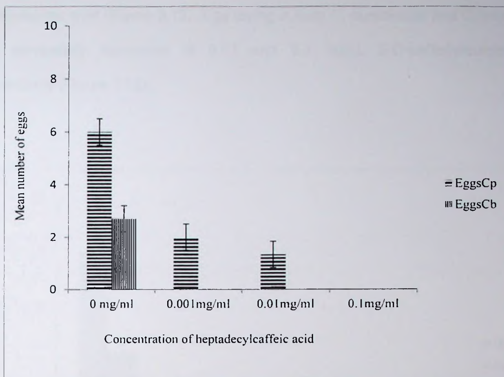
Figure 5.11. Mean number of eggs laid by C. puncticollis and C. brunneus on sweetpotato root cores treated with heptadecylcaffeic acid.
