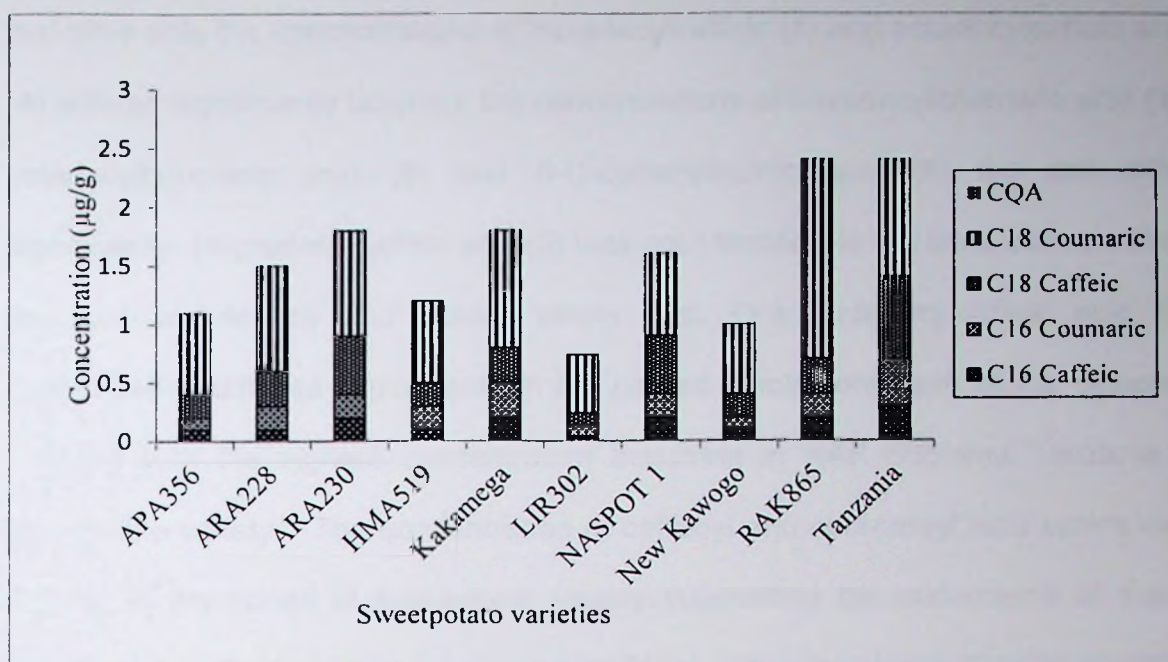
Figure 4.7 Mean concentration of hydroxycinnamic acid esters in the root flesh of sweetpotato varieties.
