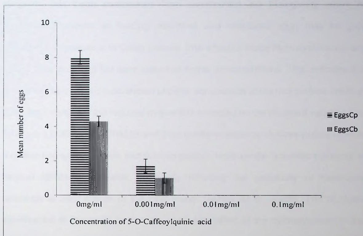
Figure 5.12. Mean number of eggs laid by C. puncticollis and C. brunneus on sweetpotato root cores treated with 5-O-caffeoylquinic acid.
