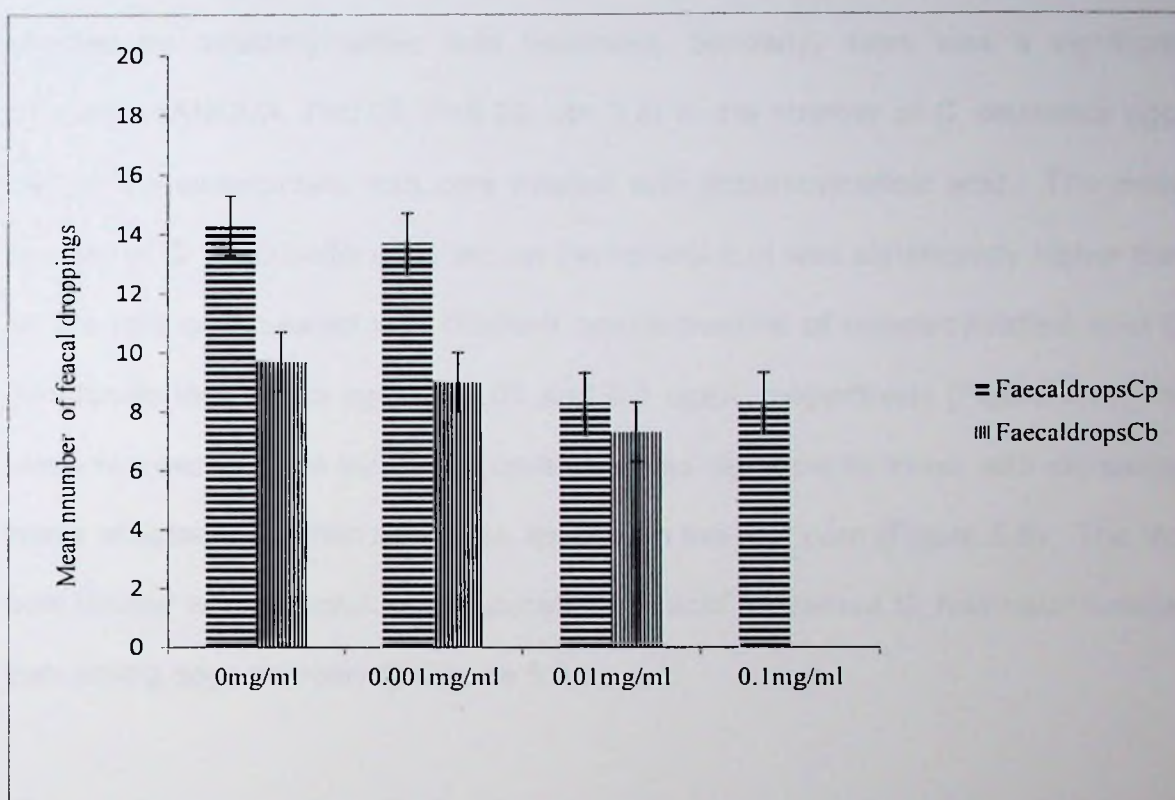
Figure 5.8. Mean number of faecal droppings produced by C. puncticollis and C. brunneus on sweetpotato root cores treated with 5-O-caffeoylquinic acid.
