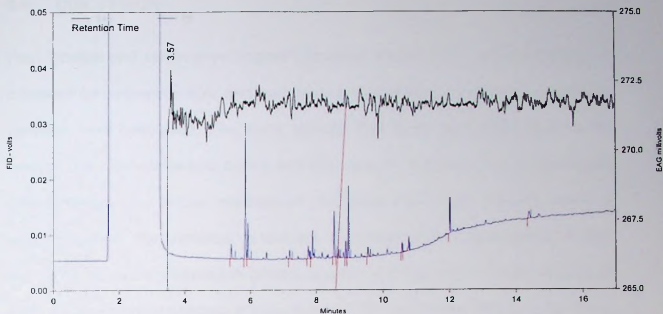
Figure 6.12. Chromatograms of New Kawogo volatiles plus pheromone and EAG response using a male C. puncticollis antenna with the tip cut and the second antenna removed
