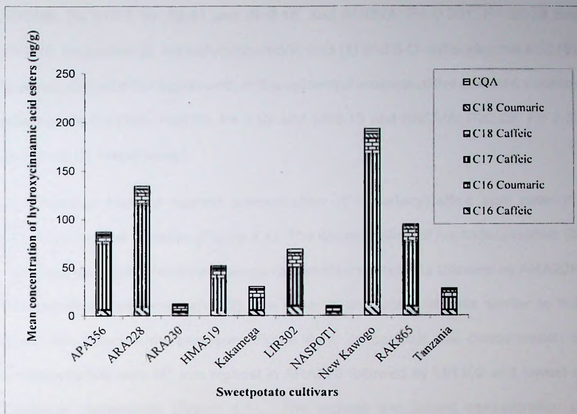
Figure 4.3 Mean concentration of hydroxycinnamic acid esters on the root peridermal tissues of selected sweetpotato varieties.
