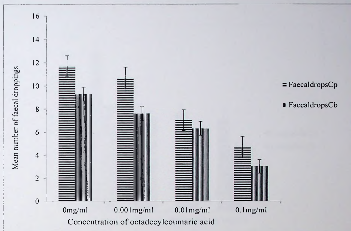
Figure 5.6. Mean number of faecal droppings produced by C. puncticollis and C. brunneus on sweetpotato root cores treated with octadecyl coumaric acid.
