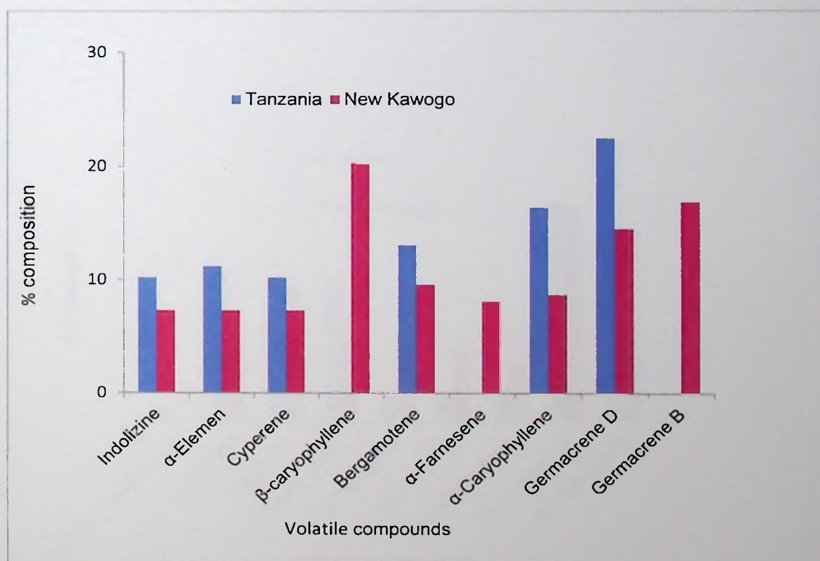
Figure 6.1. Mean percentage volatile chemical compound composition produced by the storage root of Tanzania and New Kawogo before weevil infestation
