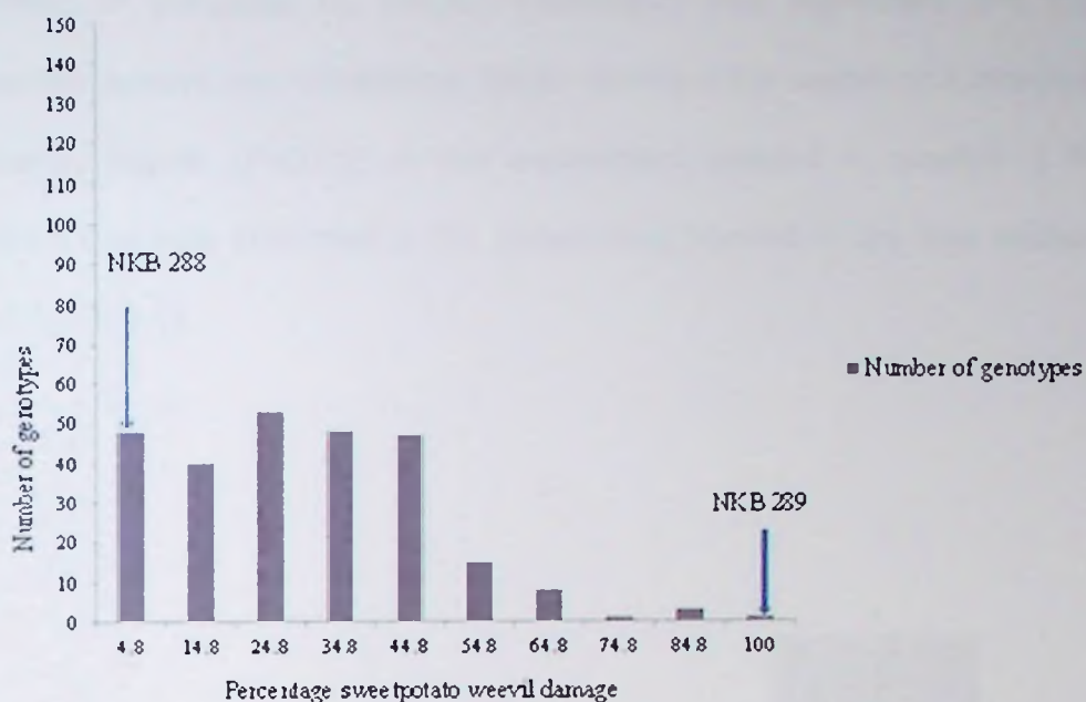
Figure 8.1. Percentage sweetpotato weevil root infestation in the segregating population of New Kawogo (NKB288) and Beauregard (NKB289).
