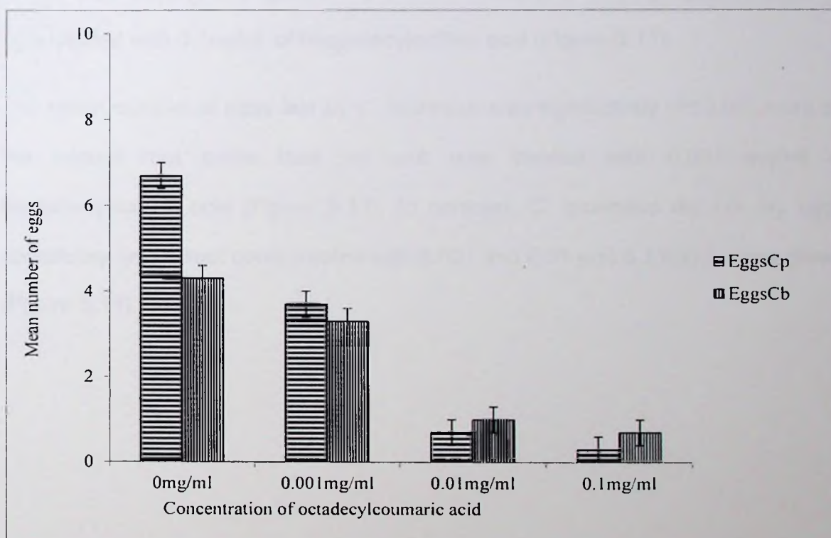
Figure 5.10. Mean number of eggs laid by C. puncticollis and C. brunneus on sweetpotato root cores treated with octadecylcoumaric acid.
