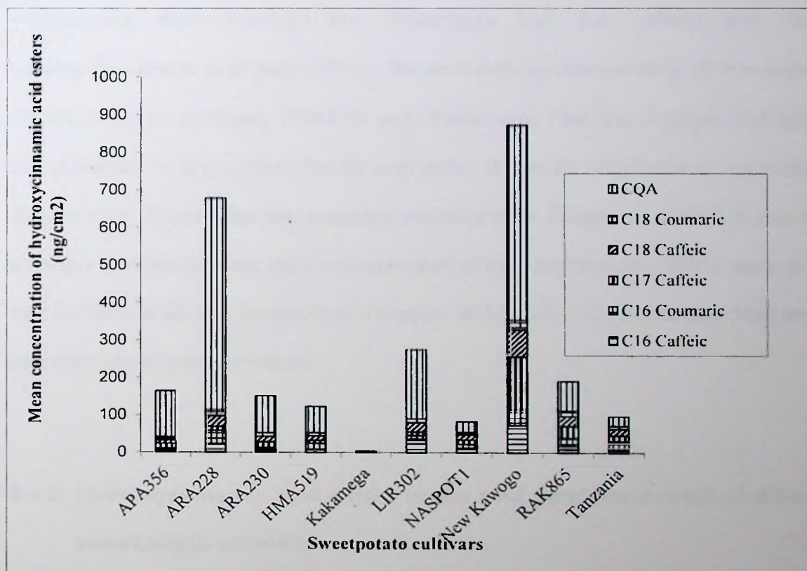
Figure 4.2. Mean concentration of hydroxycinnamic acid esters on the root surface of selected sweetpotato varieties assayed at NRI.
