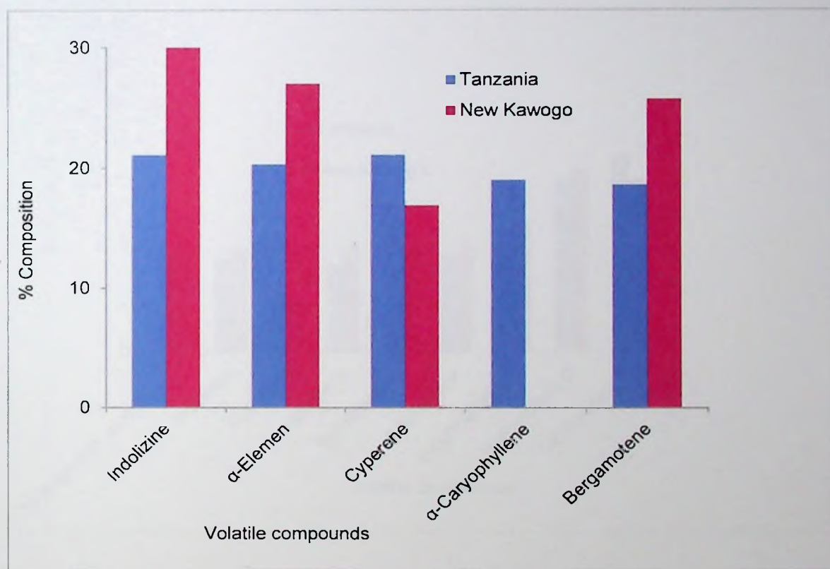
Figure 6.3. Mean percentage volatile chemical compound composition produced by the aerial parts of Tanzania and New Kawogo before weevil infestation
