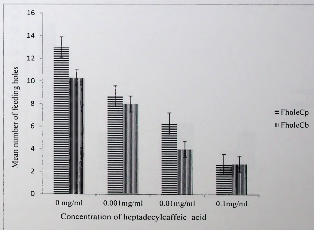
Figure 5.3. Mean number of feeding holes produced by C. puncticollis and C. brunneus on sweetpotato root plugs treated with heptadecylcaffeic acid.
