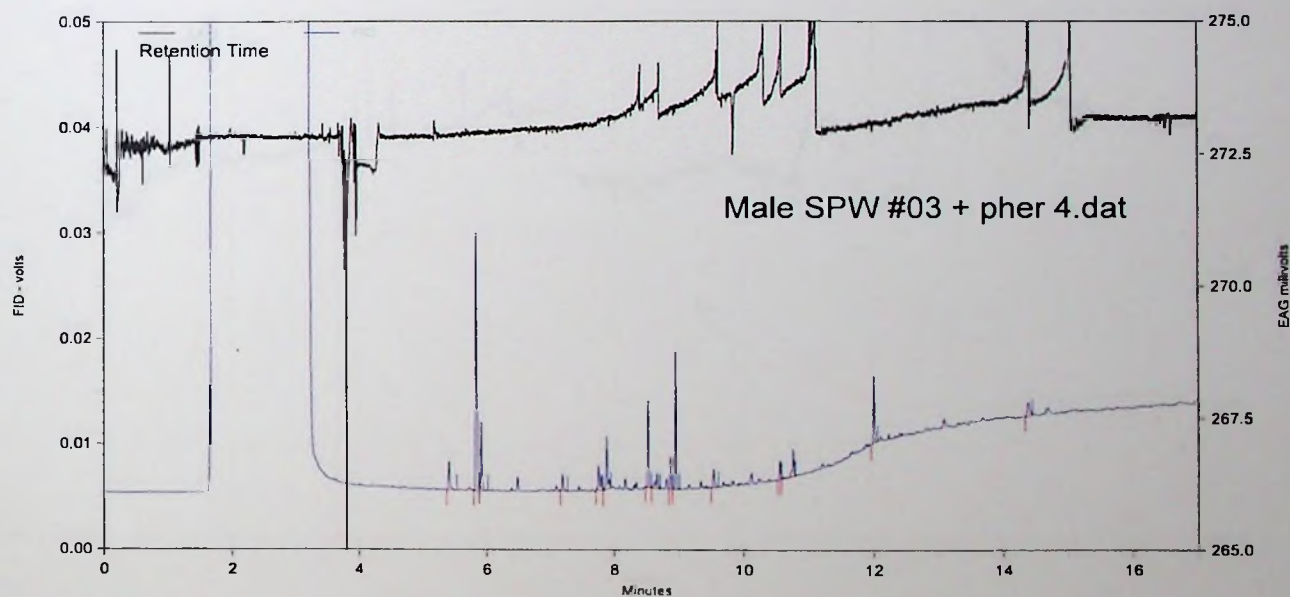
Figure 6.9. Chromatograms of Tanzania volatiles plus pheromone and EAG response using a male C. puncticollis antenna with the tip cut and the second antenna removed
